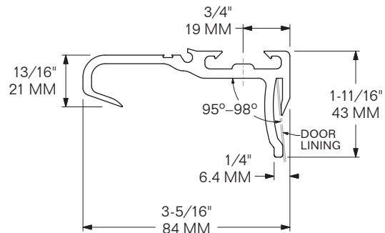
TYPICAL PROFILE (A) ALL 4 SIDES
